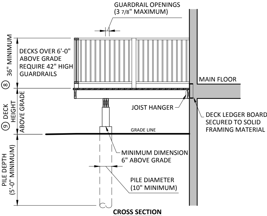
CROSS SECTION
