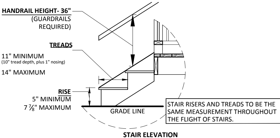
STAIR ELEVATION
