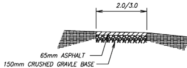
2.0m OR 3.0m PAVED PATH
