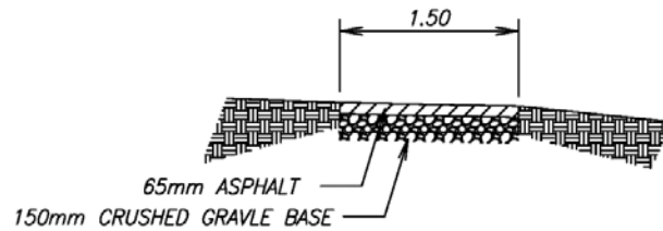
1.50m PAVED PATH
